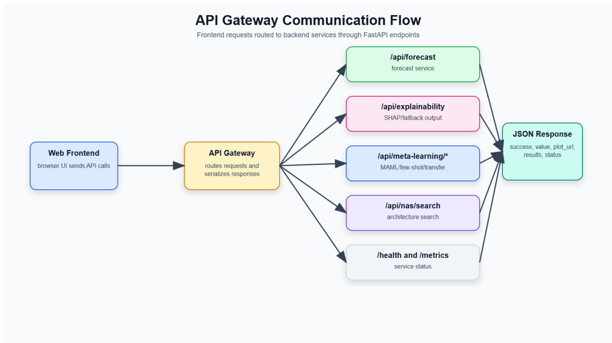
Figure 12 : API Gateway Communication Flow
