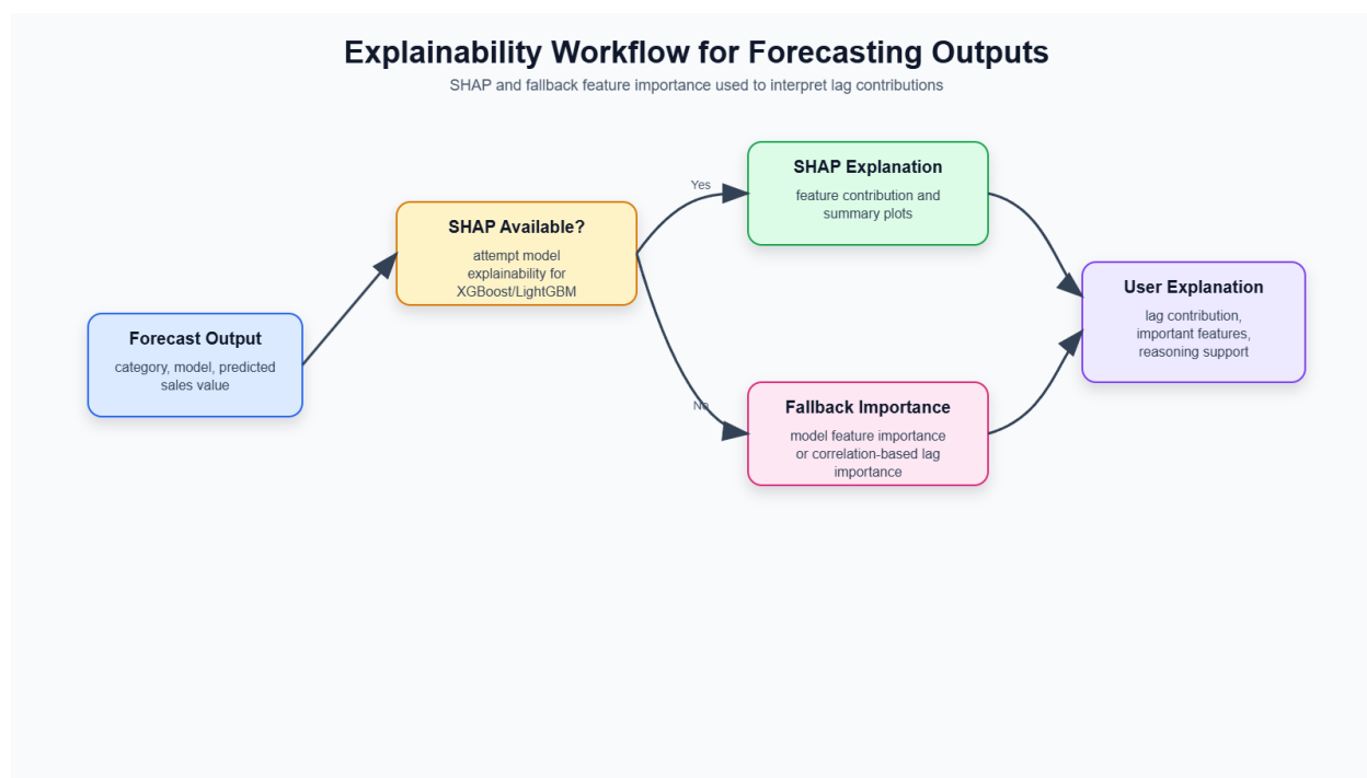
Figure 9: Explainability Workflow for Forecasting Outputs
