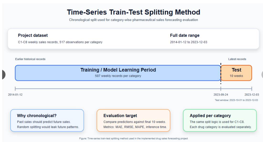
Figure 5 : Time-Series Train-Test Splitting Method
