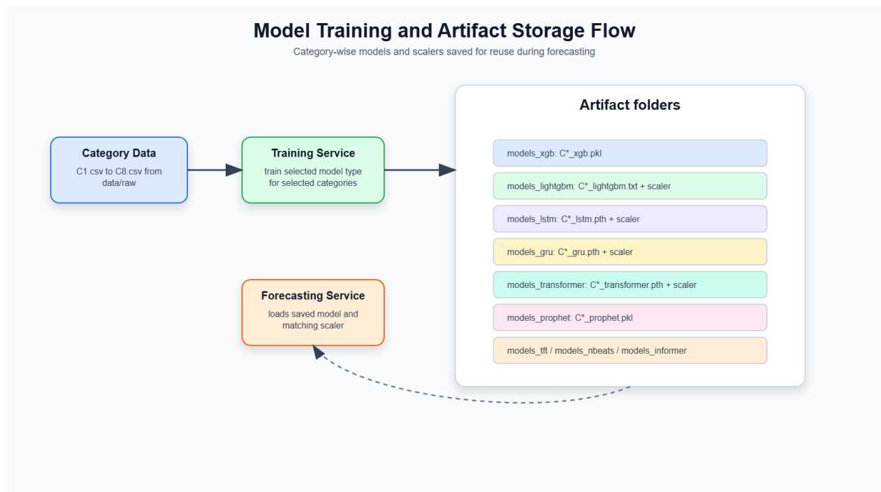
Figure 7 : Model Training and Artifact Storage Flow
