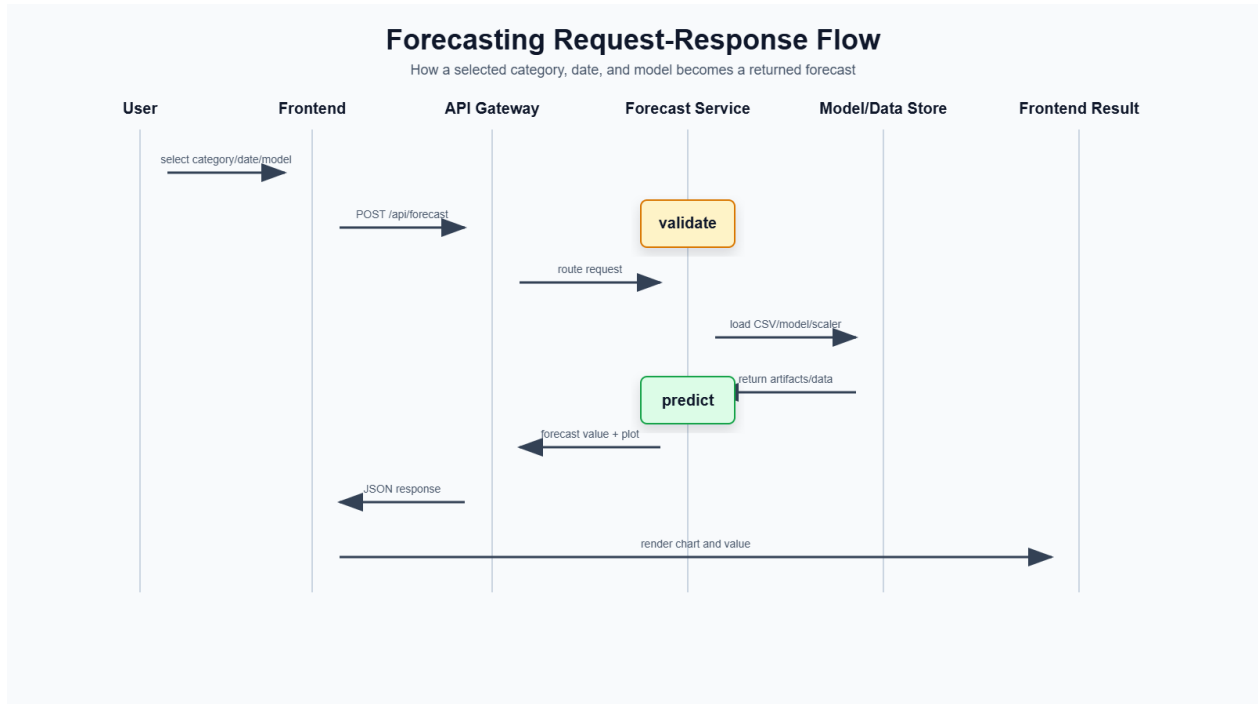
Figure 8 : Forecasting Request-Response Flow
