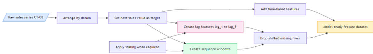
Figure 4: Time-Series Feature Engineering Process
