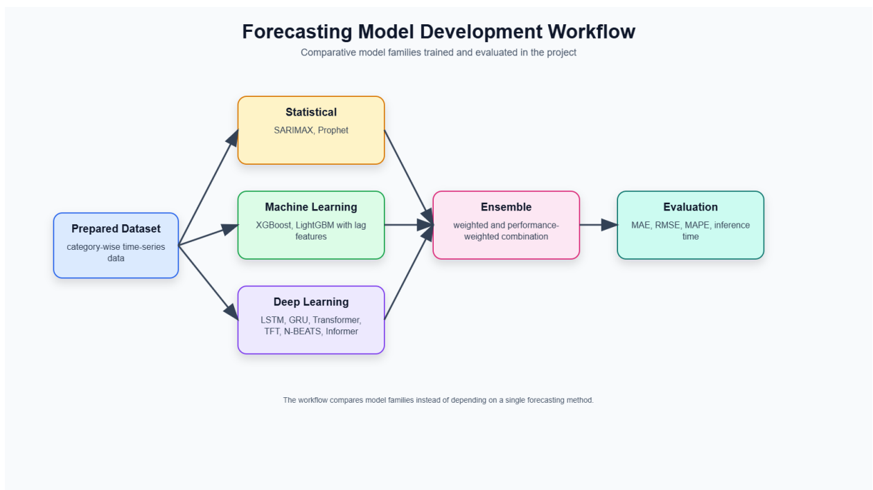
Figure 6: Forecasting Model Development Workflow
